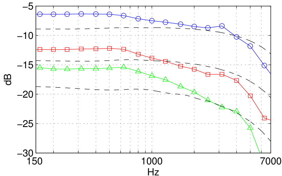
Figure 4: Transfer functions of B&K HATS from position 3.1 (MRP) to positions 1.1, 1.3, and 1.4 ( \circ , \square , and \triangle ). Corresponding modeled cases are included for the same positions.
