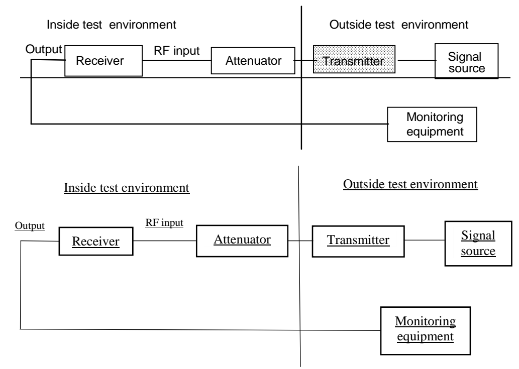
Figure 4: Test configuration for receivers
