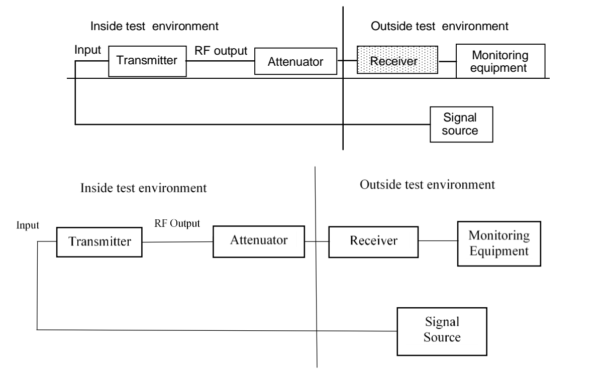
Figure 3: Test configuration for transmitters
