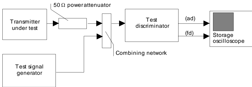
Figure 3: Measurement arrangement
