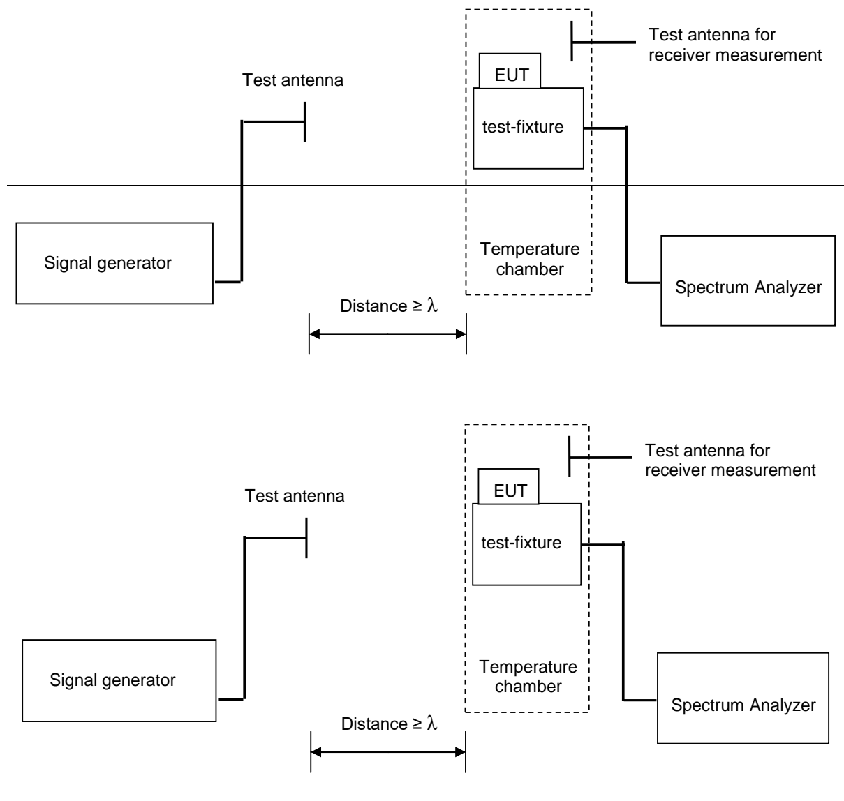
Figure 6: Validation of test set-up with EUT in place
