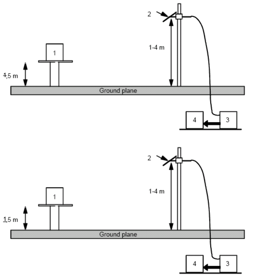
Figure BE.1: Outdoor test site
