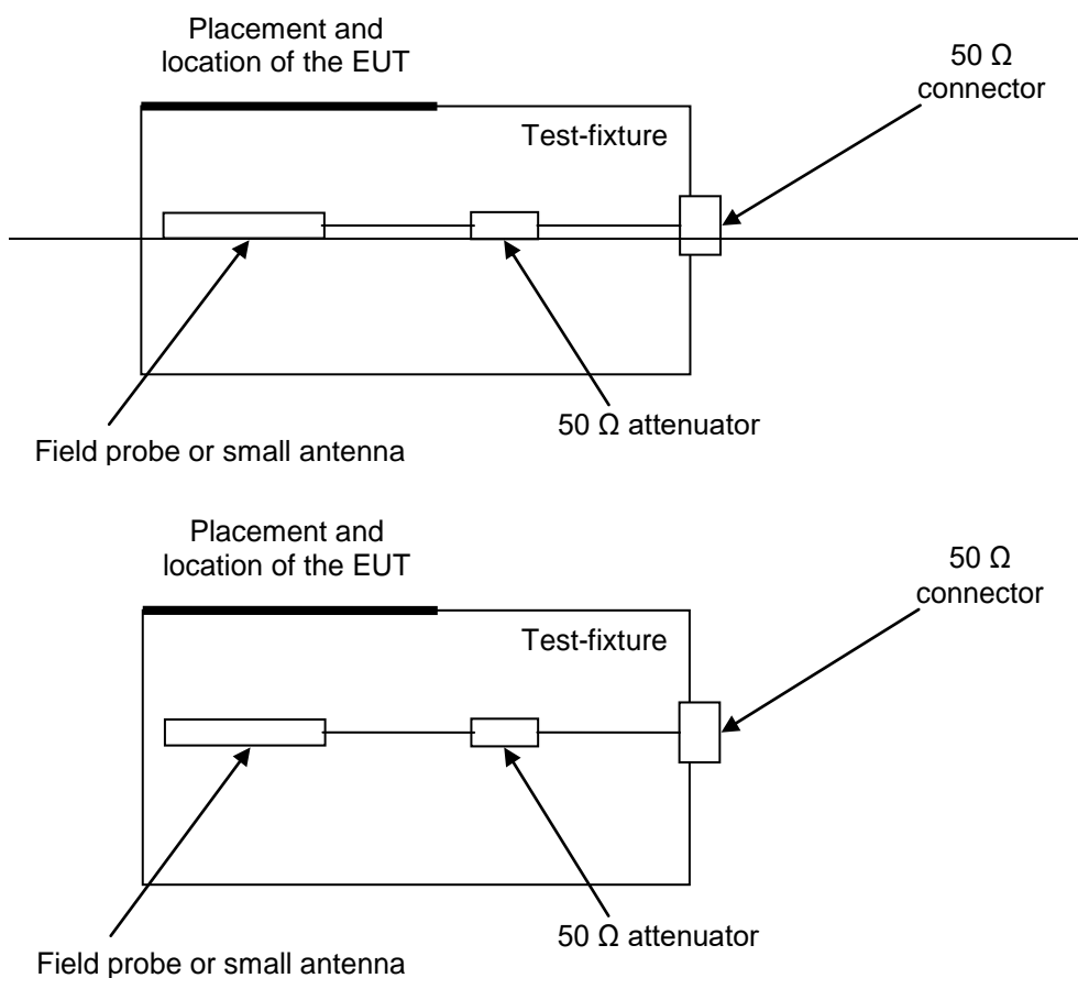
Figure 4: Test fixture
