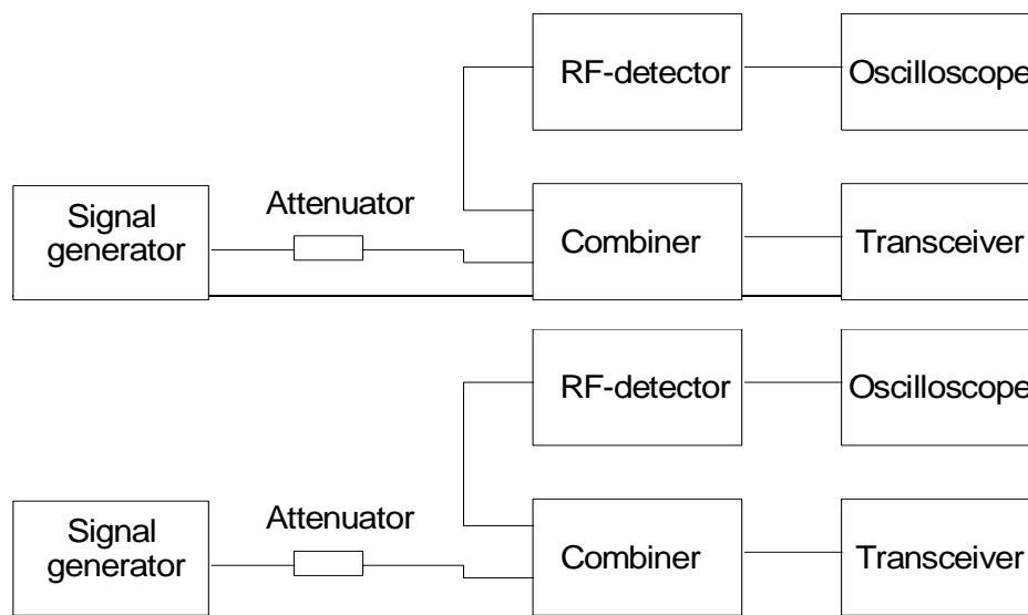
Figure 3: Measurement arrangement
