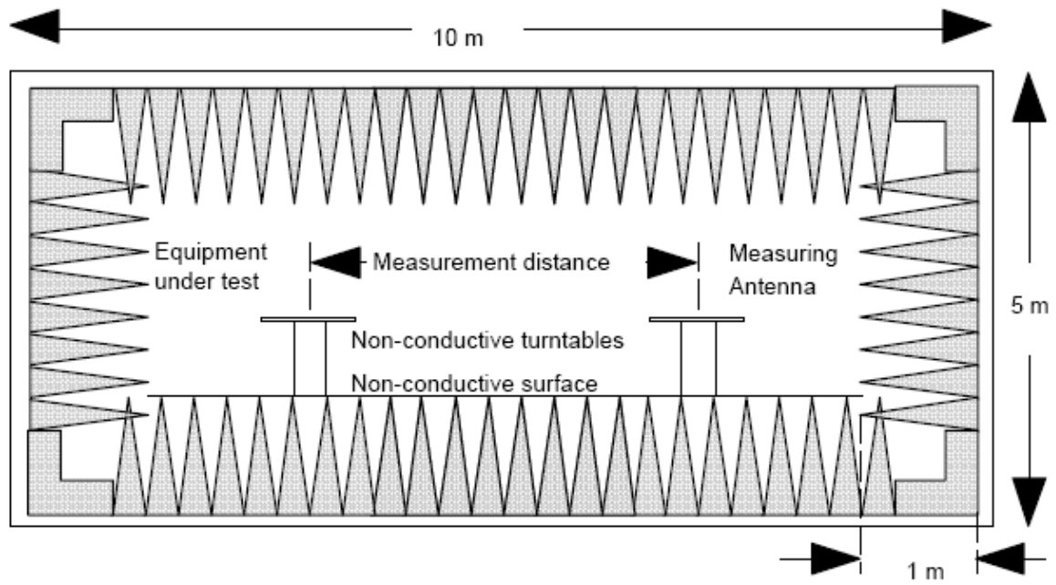
Ground plan
