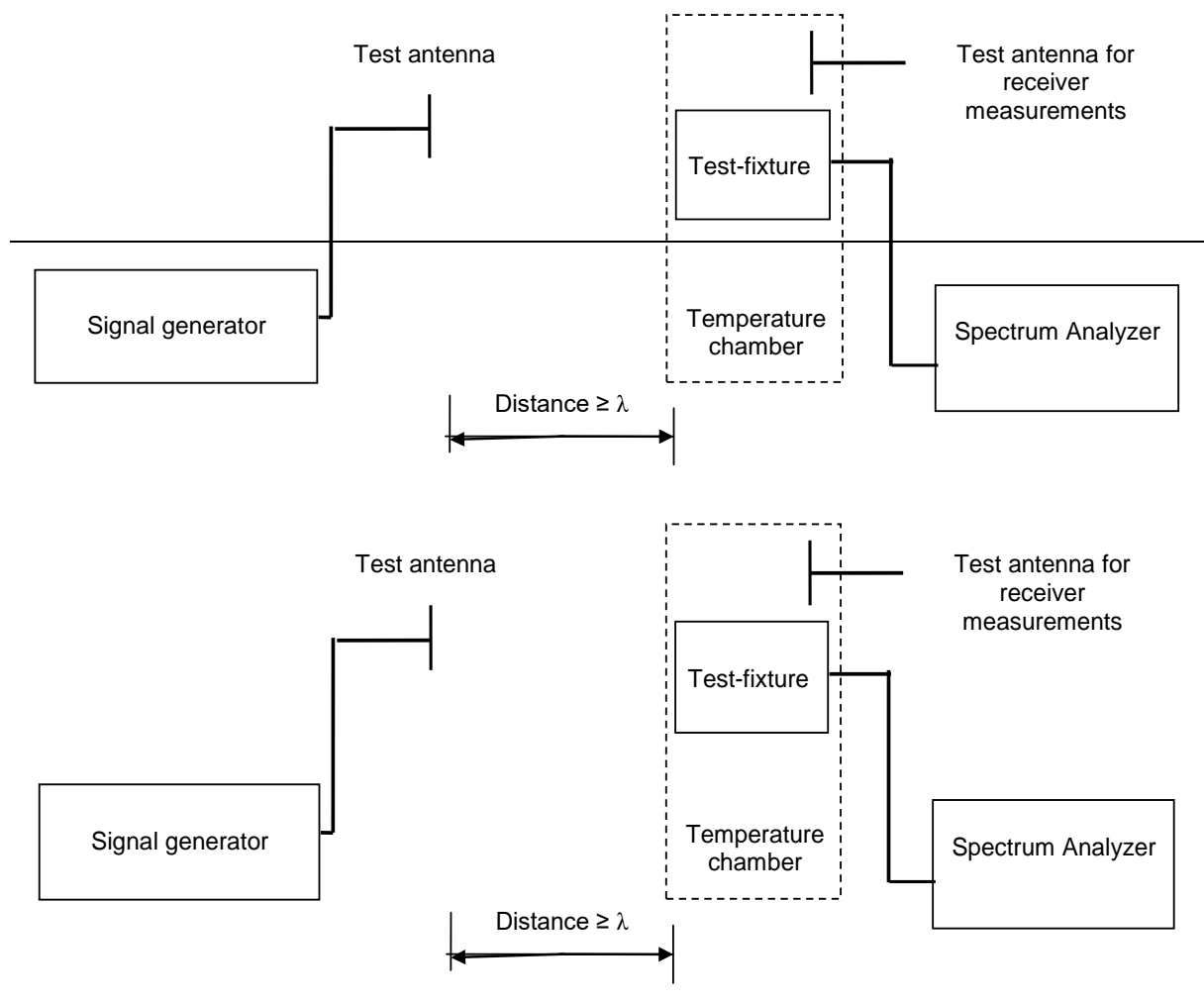
Figure 5: Validation of test set-up without EUT
