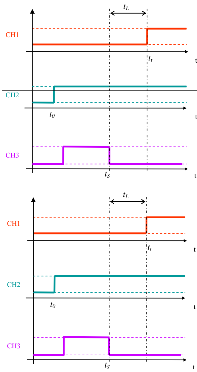
Figure F1.3: Minimum listen time after detection, t_L , measurement
