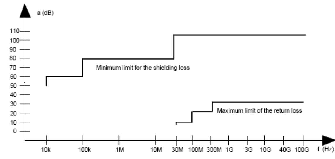
Figure BE.3: Specification for shielding and reflections
