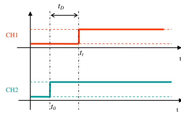
Figure F1.2: Minimum listen time, t_D , measurement
