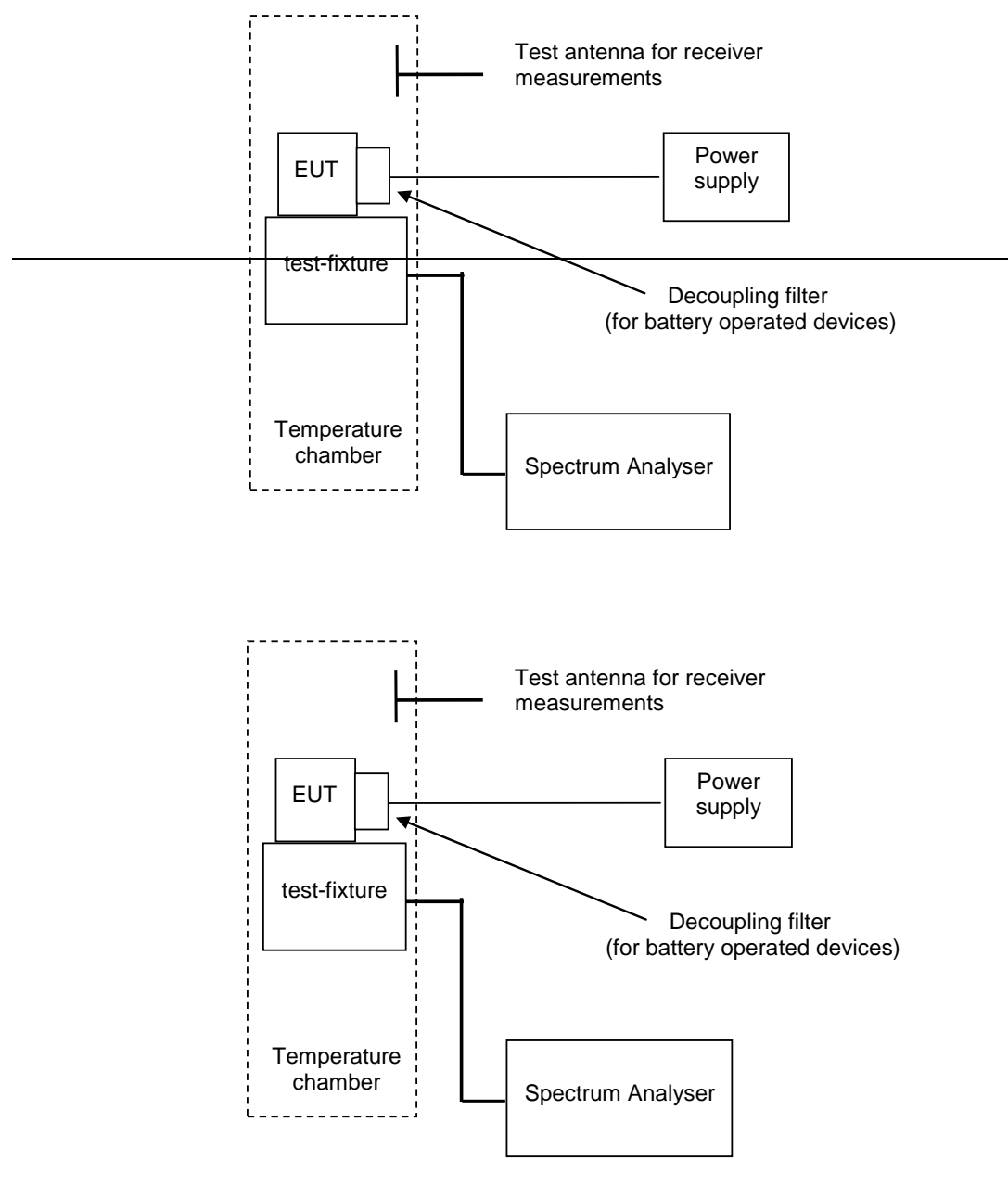
Figure 7: Test of EUT
