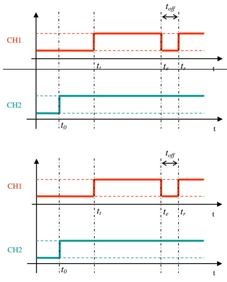
Figure F1.5: Maximum transmit off-time, t_{off} measurement
