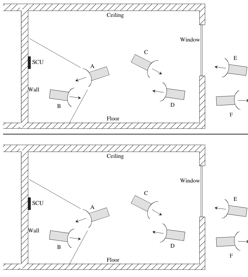
Figure EH.1: Example for RFID system with an automatic RF power control for in- and outside building operation
