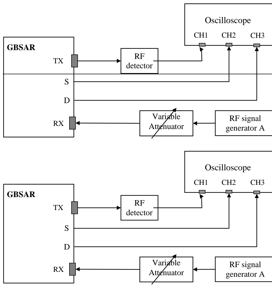
Figure 4.1: DAA measurement arrangement
