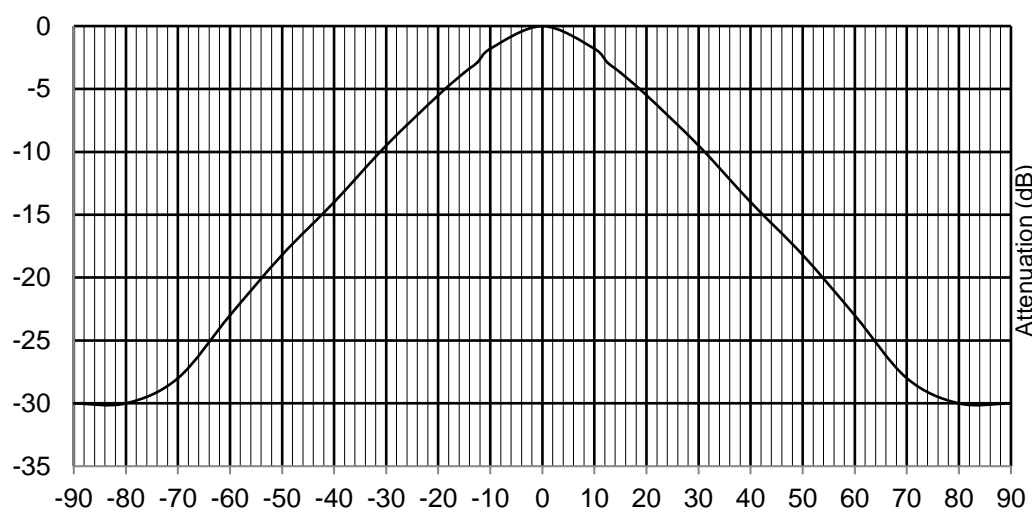
Figure 7: Minimum attenuation of the vertical antenna pattern
