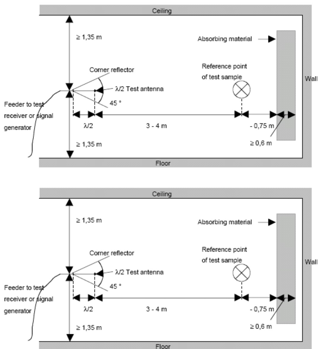
Figure BE.2: Indoor site arrangement (shown for horizontal polarization)
