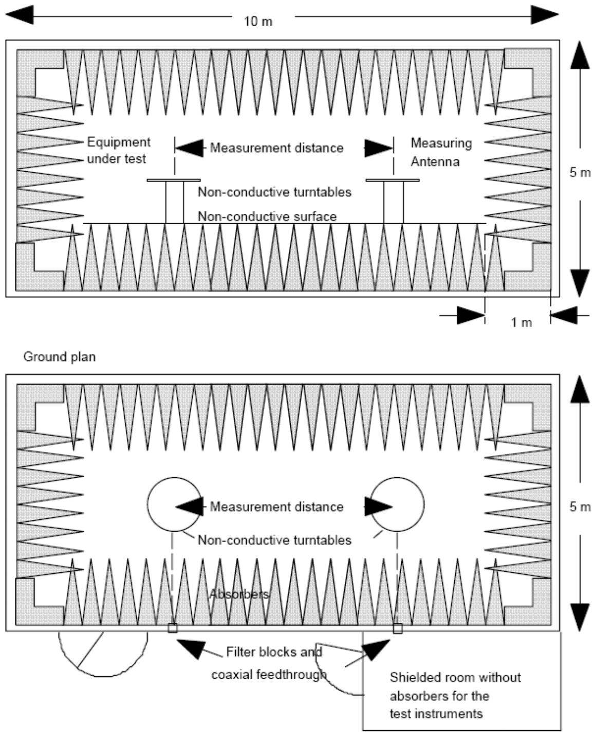
Figure BE.4: Example of construction of an anechoic shielded chamber
