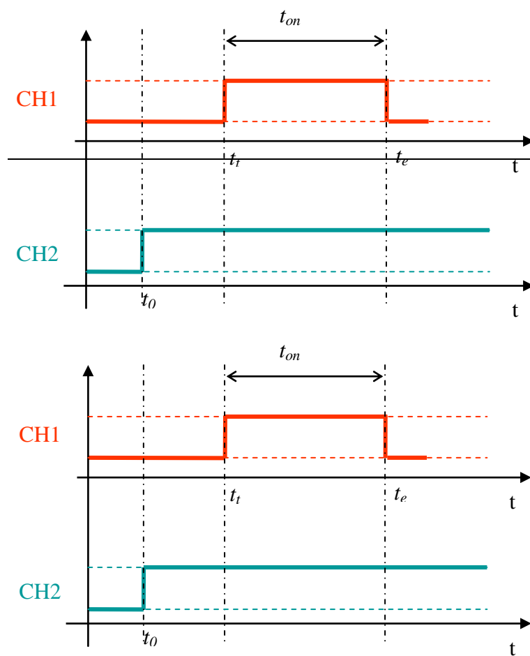
Figure 4: Maximum transmit on-time, t_{on} , measurement
