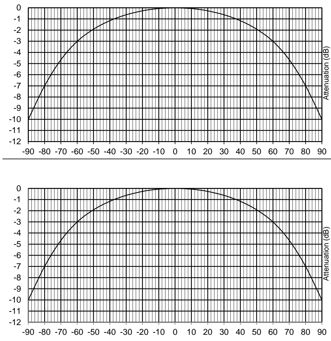
Figure F.8: Minimum attenuation of the horizontal antenna pattern
