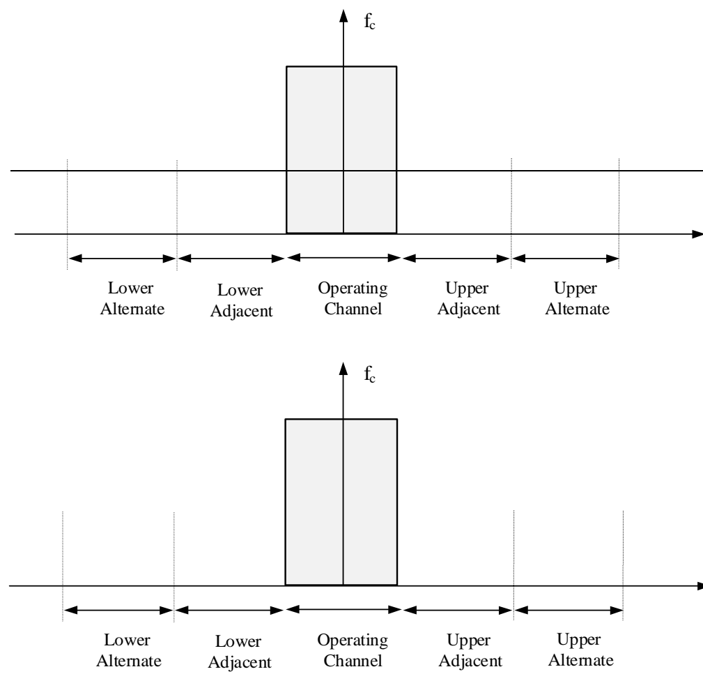
Figure 1: Adjacent and alternate adjacent channel definitions
