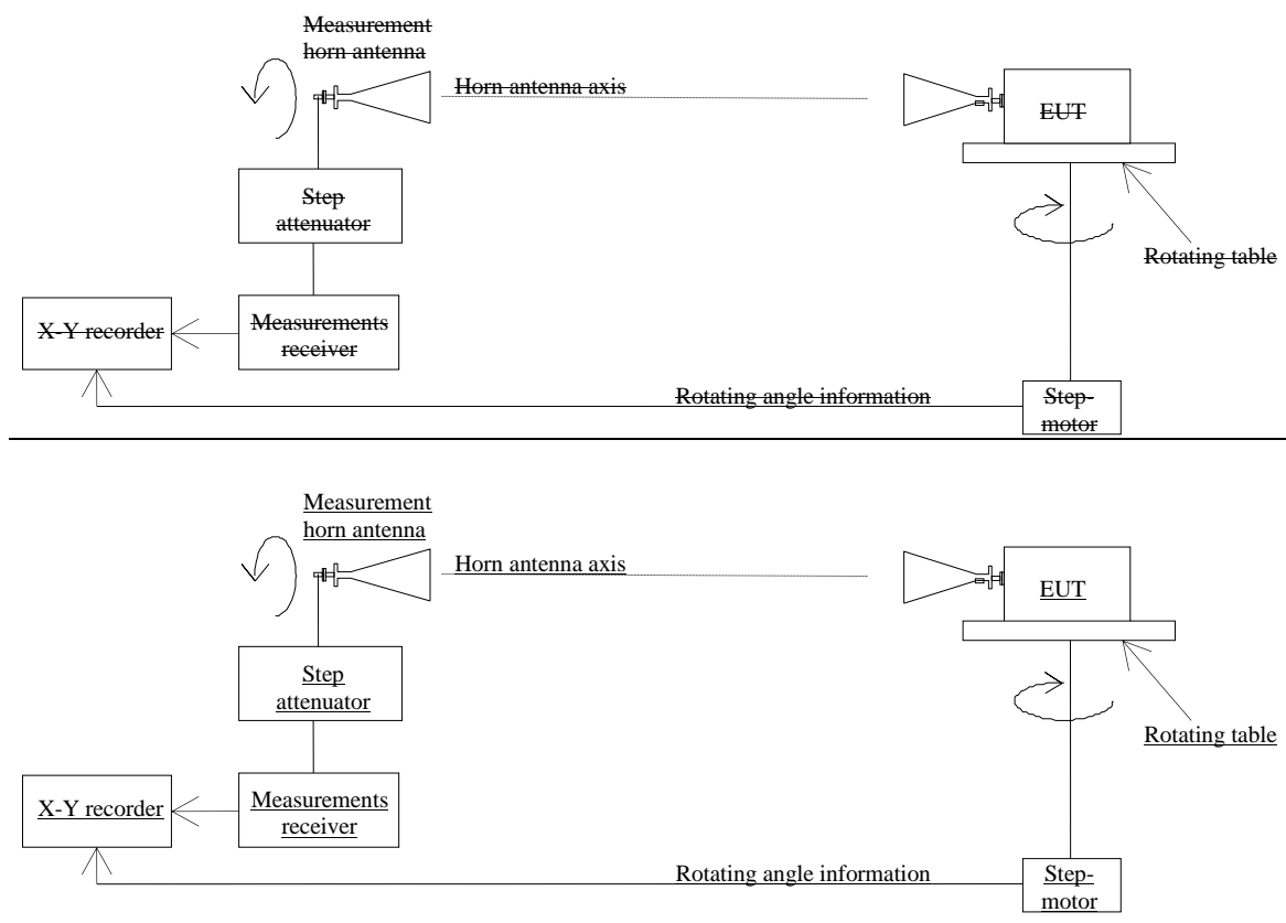
Figure F1.6: Test set-up for measurement of antenna pattern
