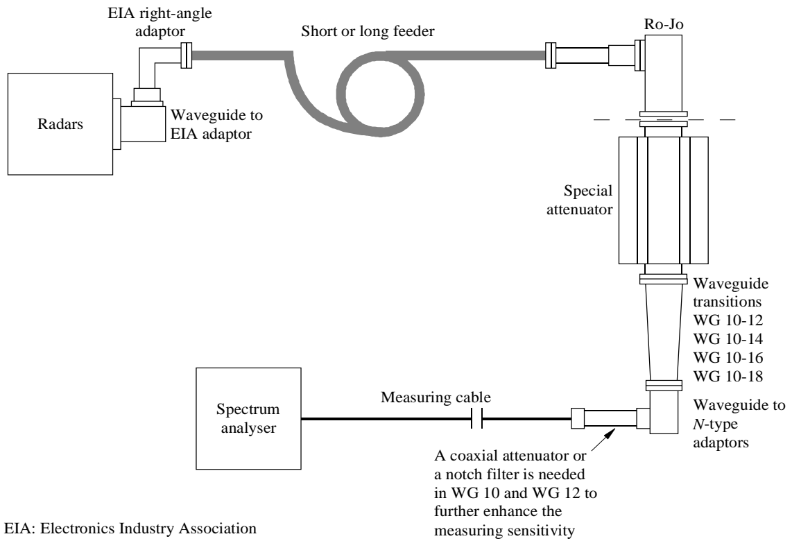
Figure CB.1: Measurement at the Ro-Jo port
