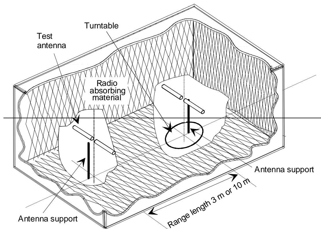
Figure B.1: A typical anechoic chamber
