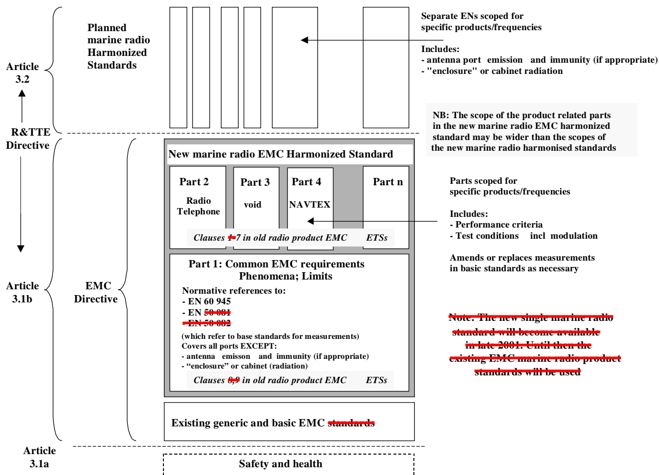
Figure 2: The new radio EMC harmonized standard
