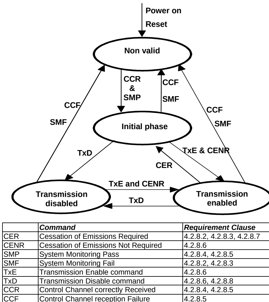
Figure 2: State transition diagram of the control and monitoring function of a NEST
