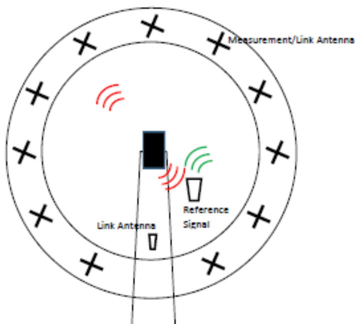
Figure B.7: Typical NTF measurement setup
