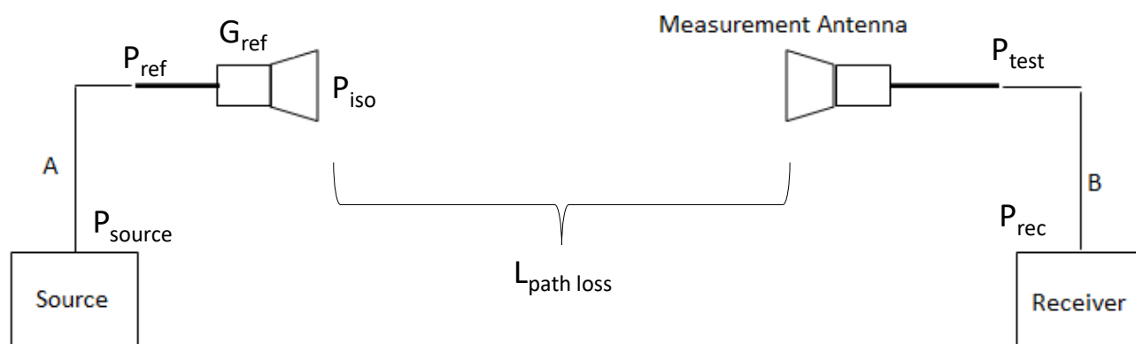
Figure B.8: NTF - Typical setup for path loss measurement
