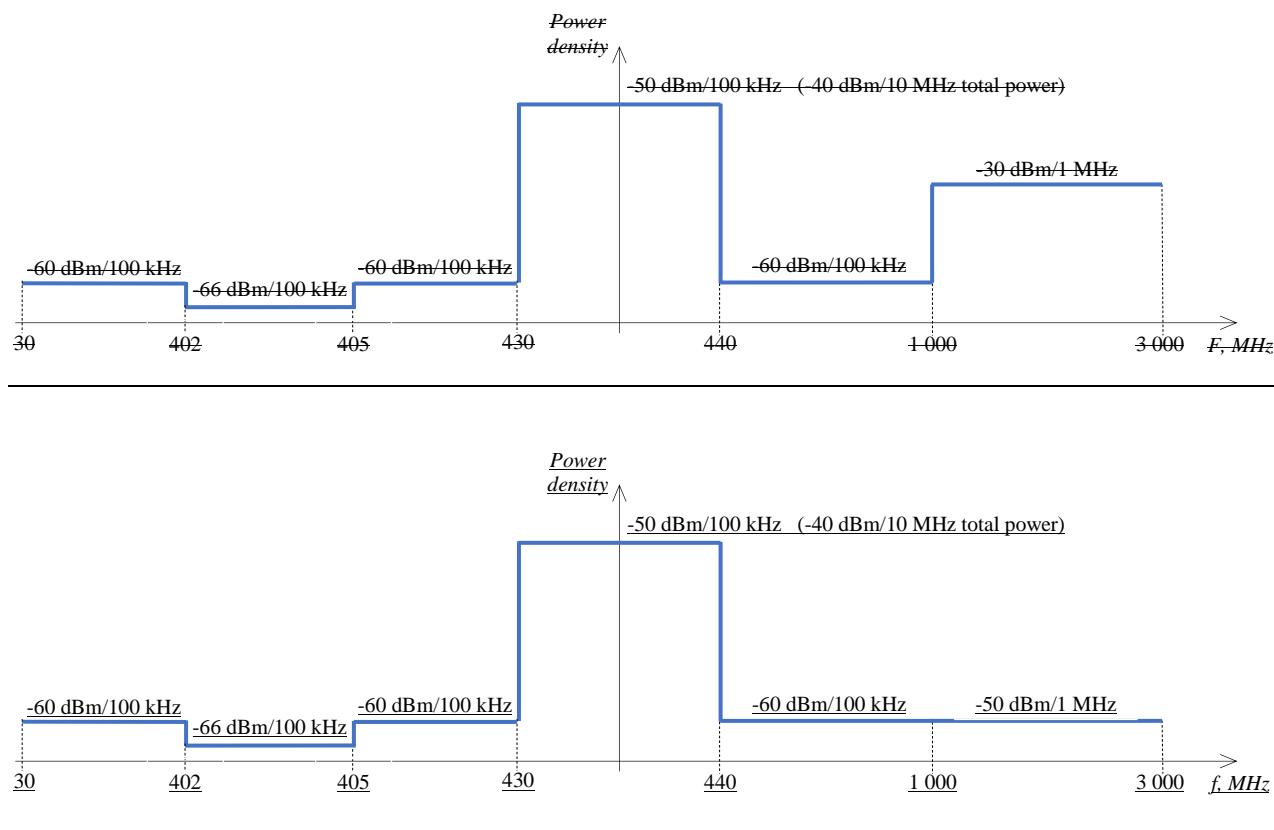
Figure 1: CCam TX emissions mask (not to scale)
