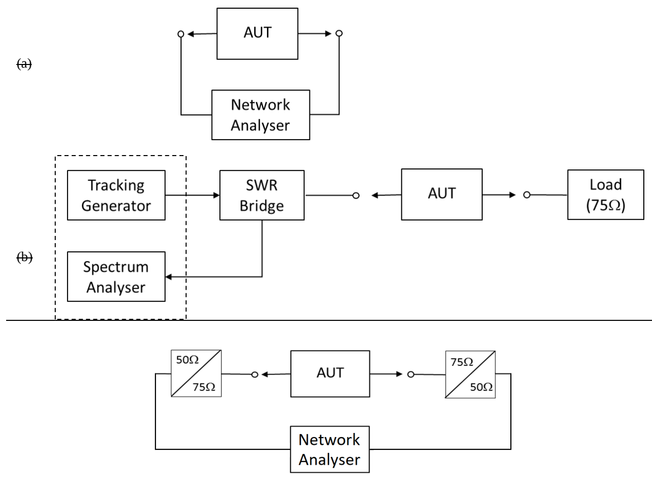
Figure 9: Return loss measurement arrangements using either a network analyser (a) or a spectrum analyser and an external bridge (b)
