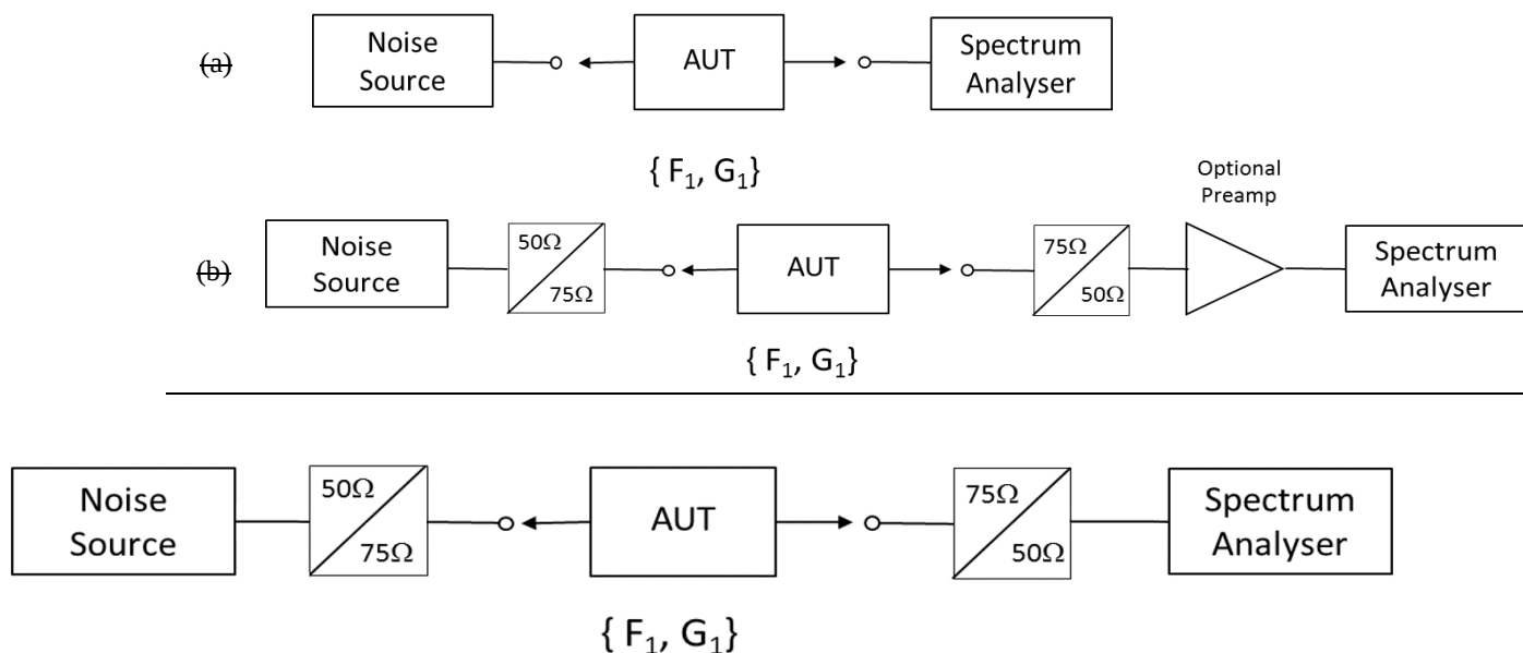
Figure 6: Measurement arrangements for noise figure test
