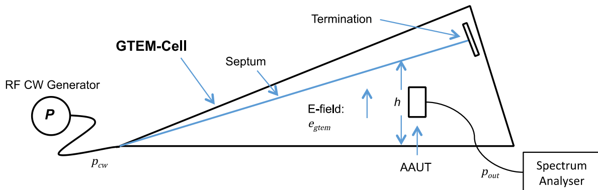
Figure 11: Active antenna gain test arrangement
