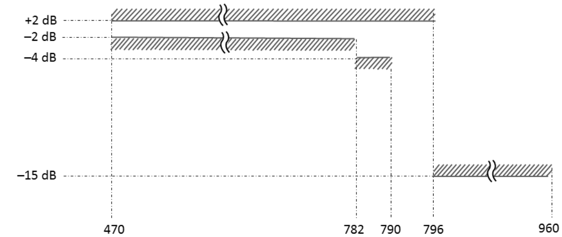
Figure 4: Adjacent band selectivity limits (classification 4) Void
