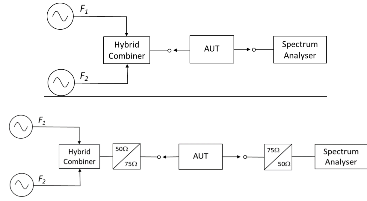
Figure 7: Measurement arrangement for intermodulation test
