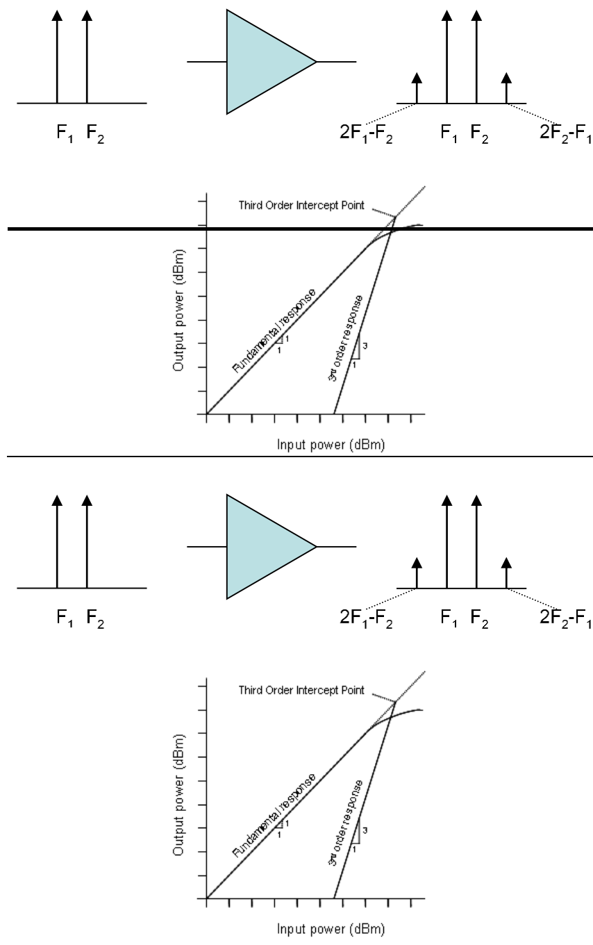
Figure 8: Third order IMD illustration
