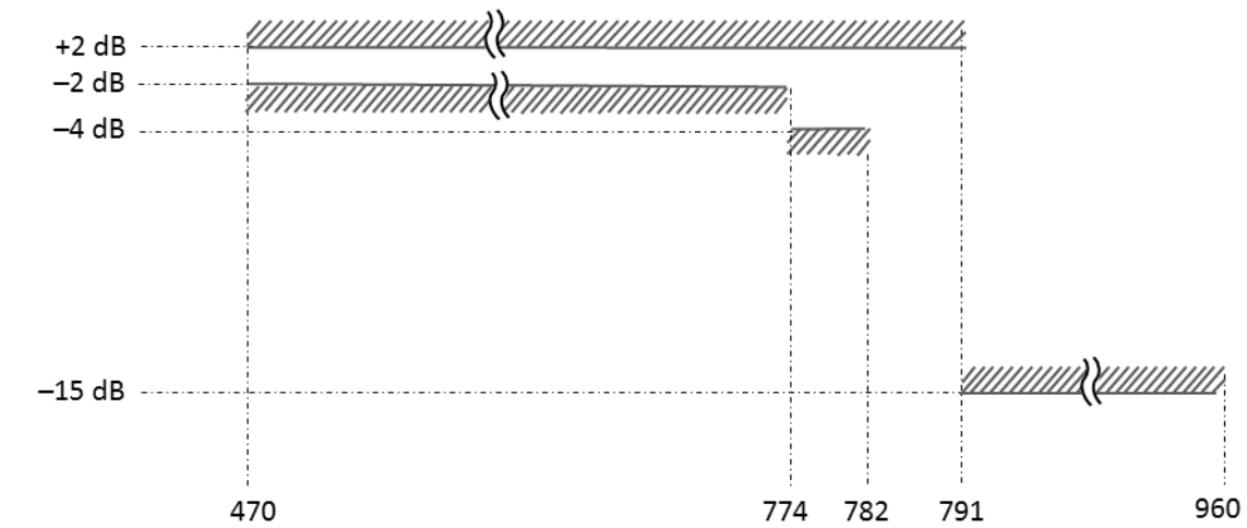
Figure 3: Adjacent band selectivity limits (classification 3) Void
