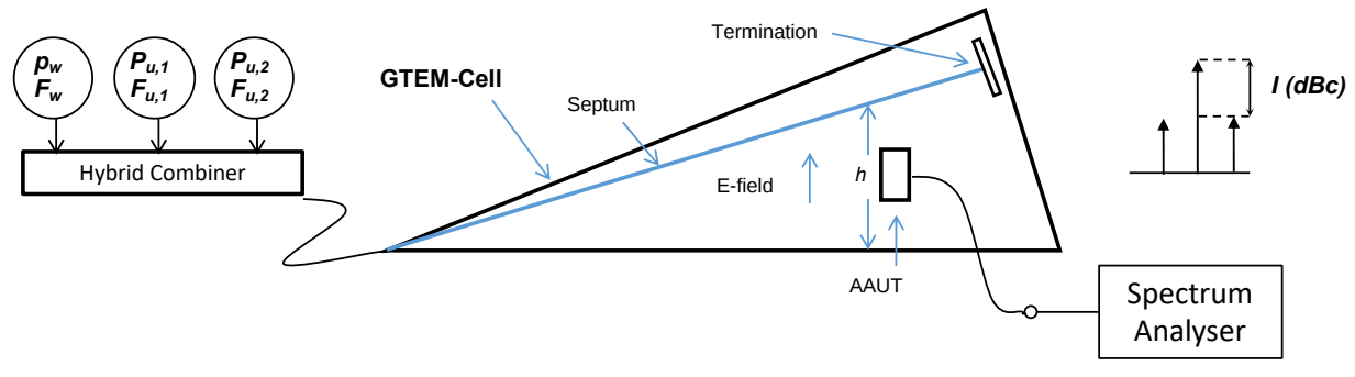
Figure 13: Active antenna immunity test arrangement
