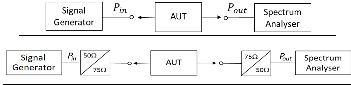
Figure 10: Amplifier frequency response measurement test arrangement
