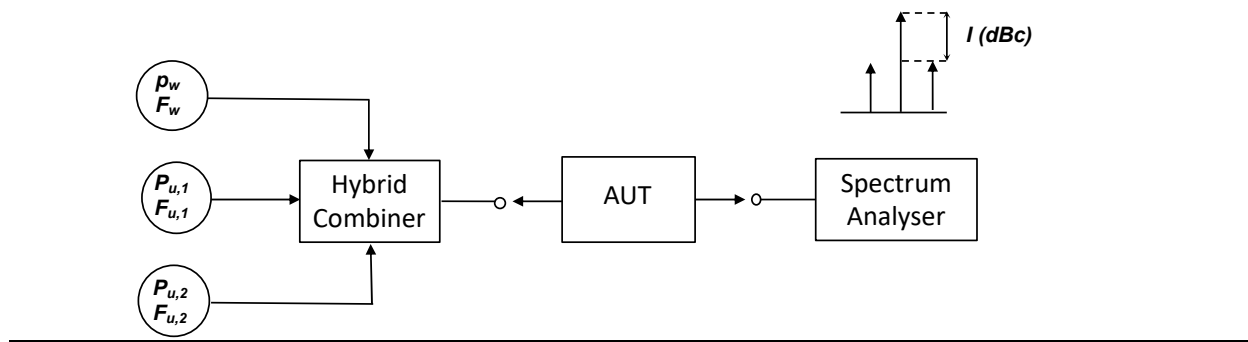
Figure 14: Amplifier immunity test arrangement
