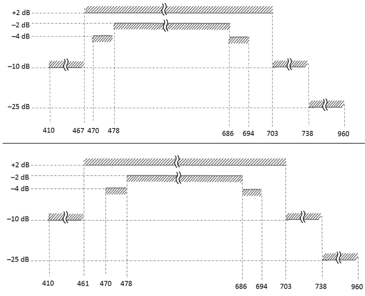
Figure 2: Adjacent band selectivity limits (classification 2)
