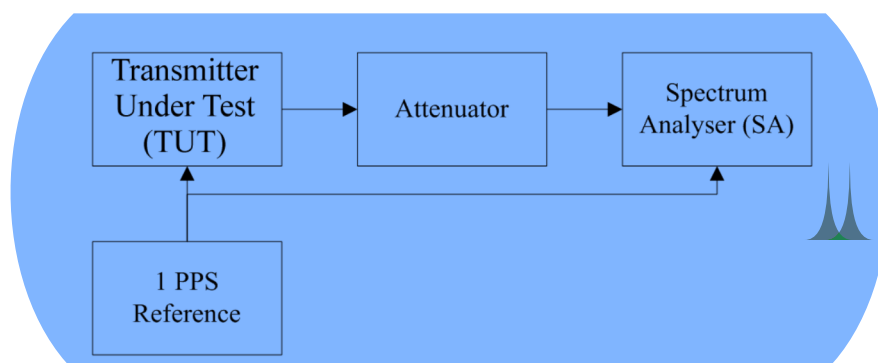
Figure 6: RF power rise and release time measurement (also applicable for RF power release time measurements and emissions in unassigned time slots measurements)
