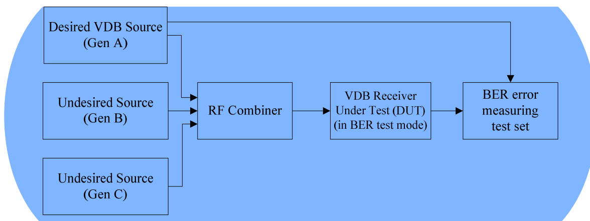
Figure 10: In band Intermodulation measurement
