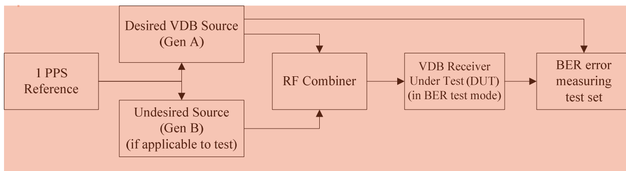
Figure 9: Time slot decoding measurement
