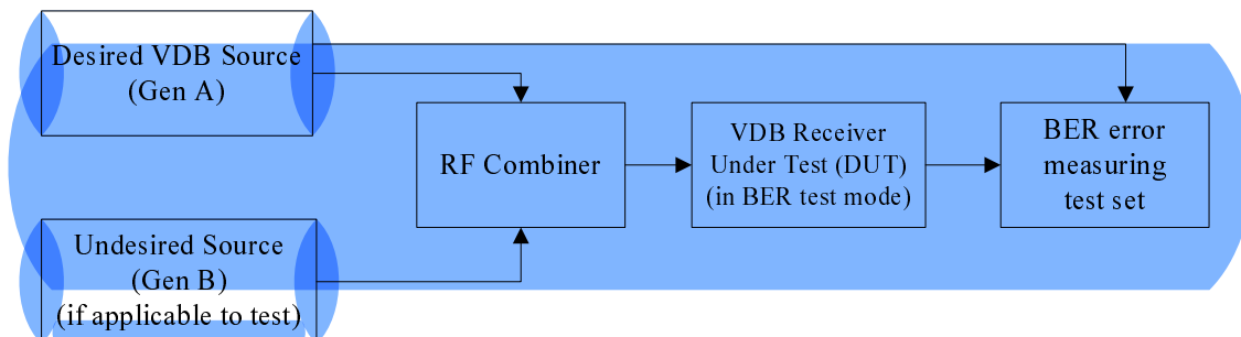
Figure 8: Receiver BER measurement
