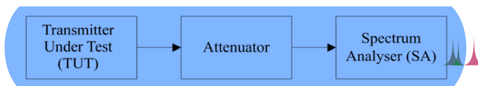
⚠⚠ Figure 2: Output power measurement
