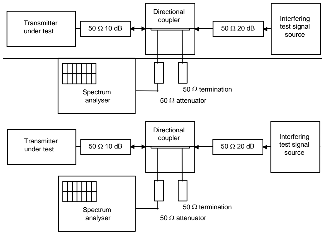
Figure 5: Measurement arrangement
