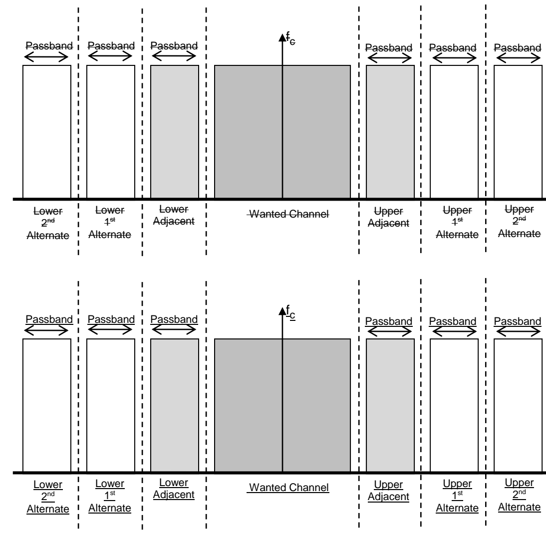
Figure 3: Adjacent and alternate channel definitions
