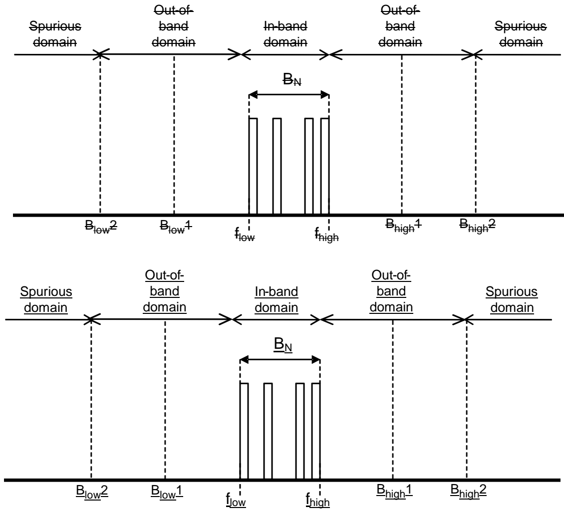
Figure 4: Unwanted Emissions Boundaries
