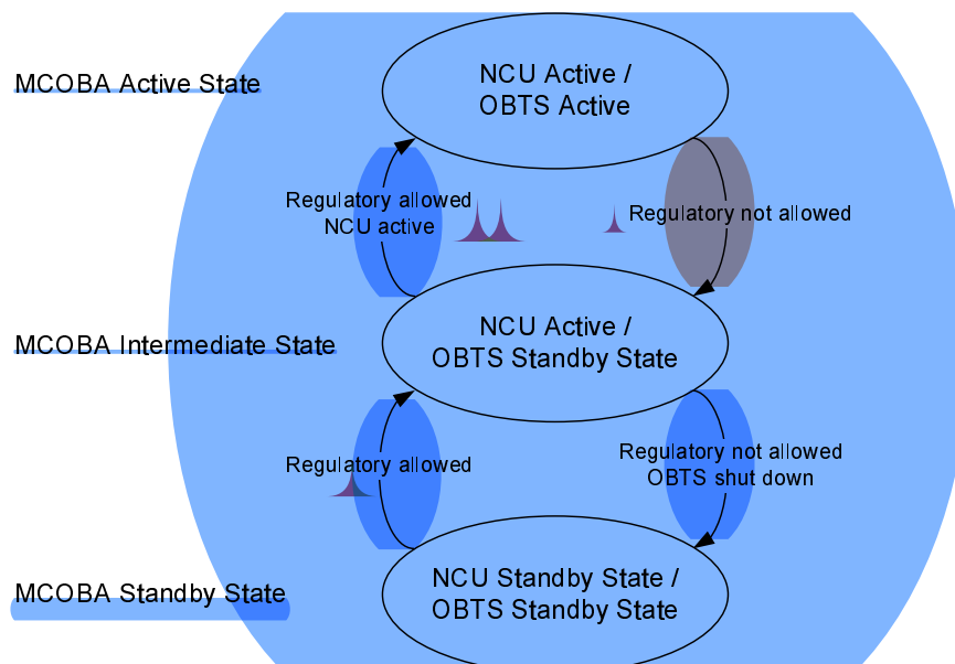
Figure 4.1.2-1: State diagram of an MCOBA system which includes an NCU
