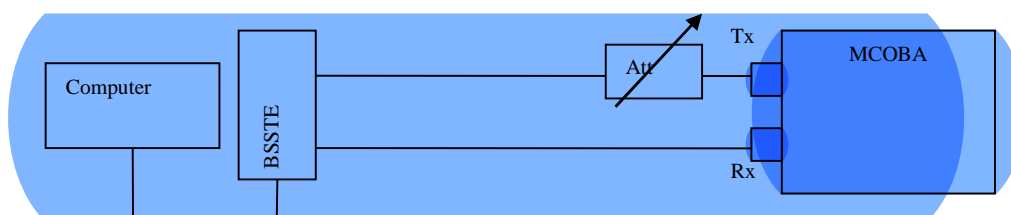
Figure 5.2.2.1.2-1: UTRA-OBTS Measurement Setup
