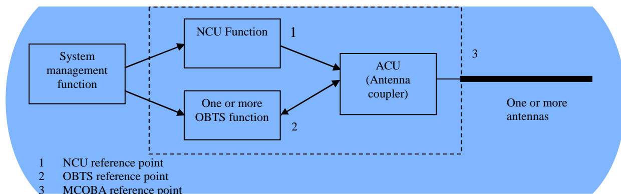
Figure 5.1.3-1: System reference points
