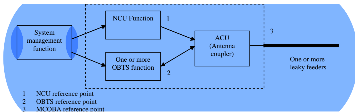
Figure C-2: System description
