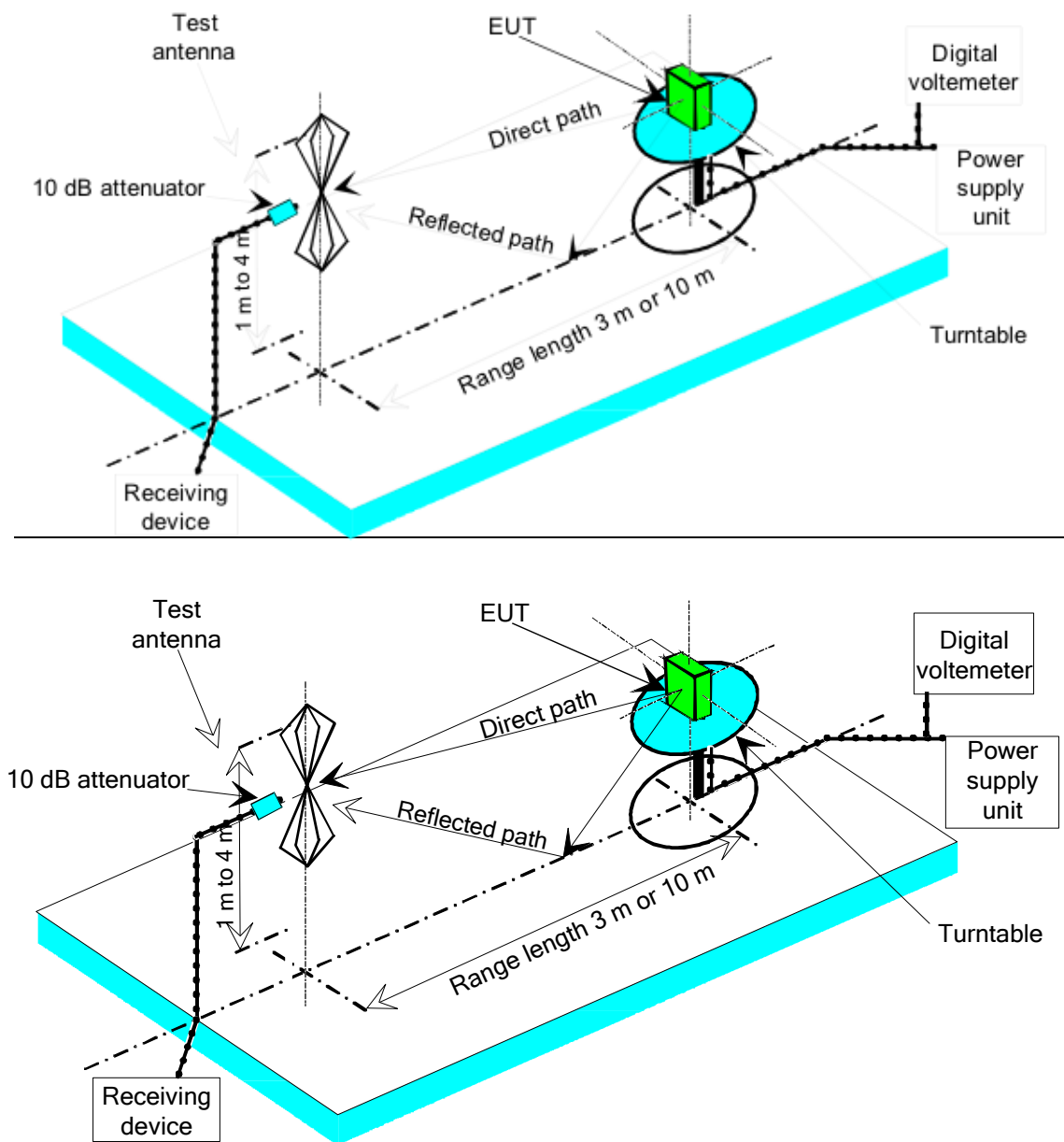
Figure B.4: Measuring arrangement on ground plane test site (OATS set-up for spurious emission testing)
