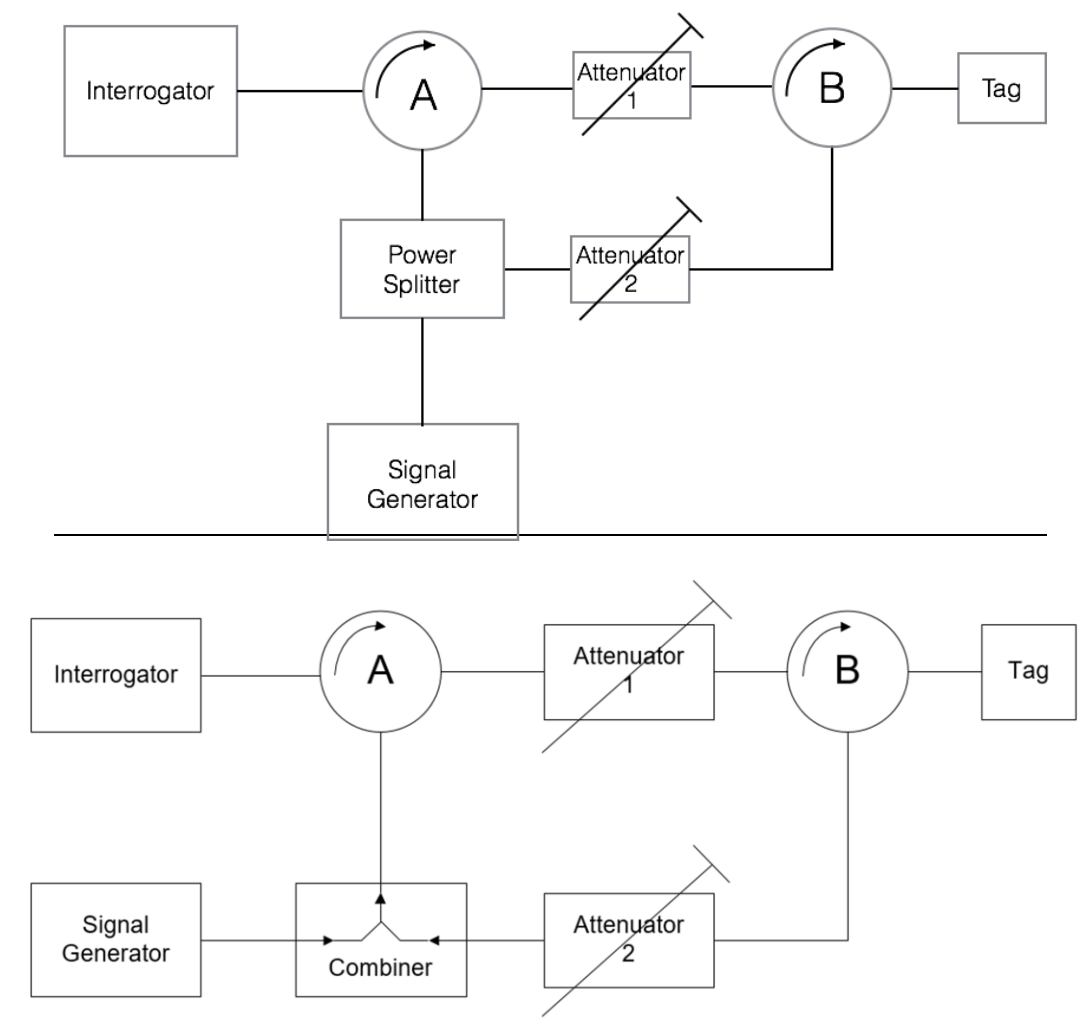
Figure 15: Conducted test set up for adjacent channel selectivity
