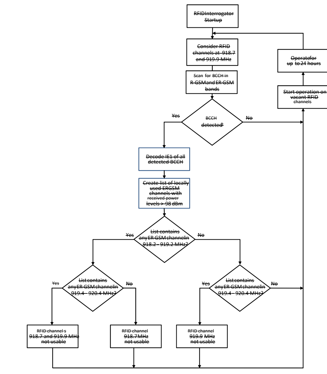
Figure C.1: GSM-R Downlink detection for ER-GSM band and RFID DAA process
