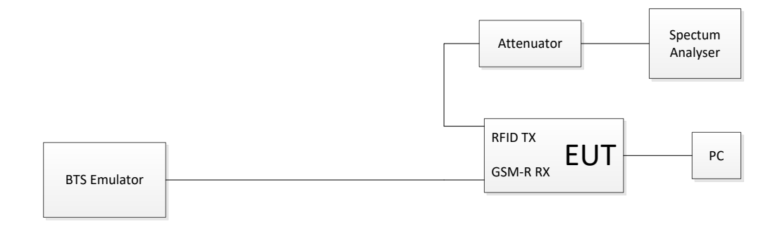
Figure 13: Set-up of equipment for mitigation test
