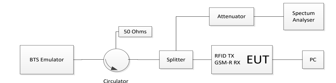
Figure 12: Set-up of equipment for mitigation test using splitter
