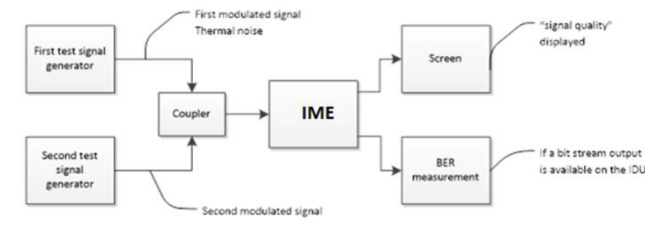
Figure 18: Test set-up for adjacent signal selectivity
