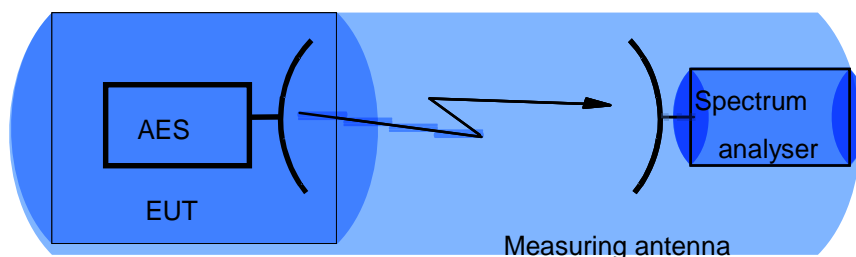
Figure 10: Test arrangement - radiated power density measurement
