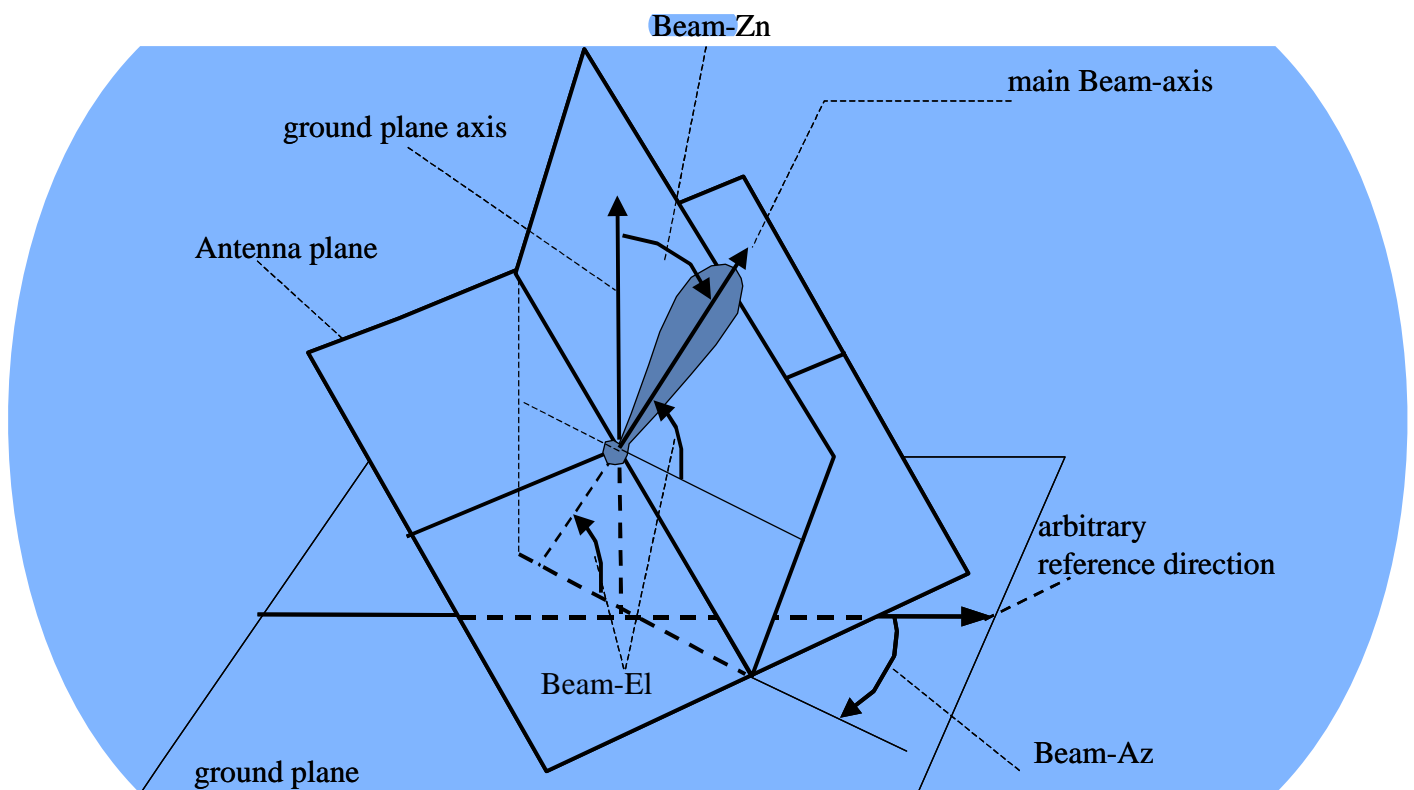
Figure 1b: Reference angles and planes for a passive (e.g. reflector) antenna
