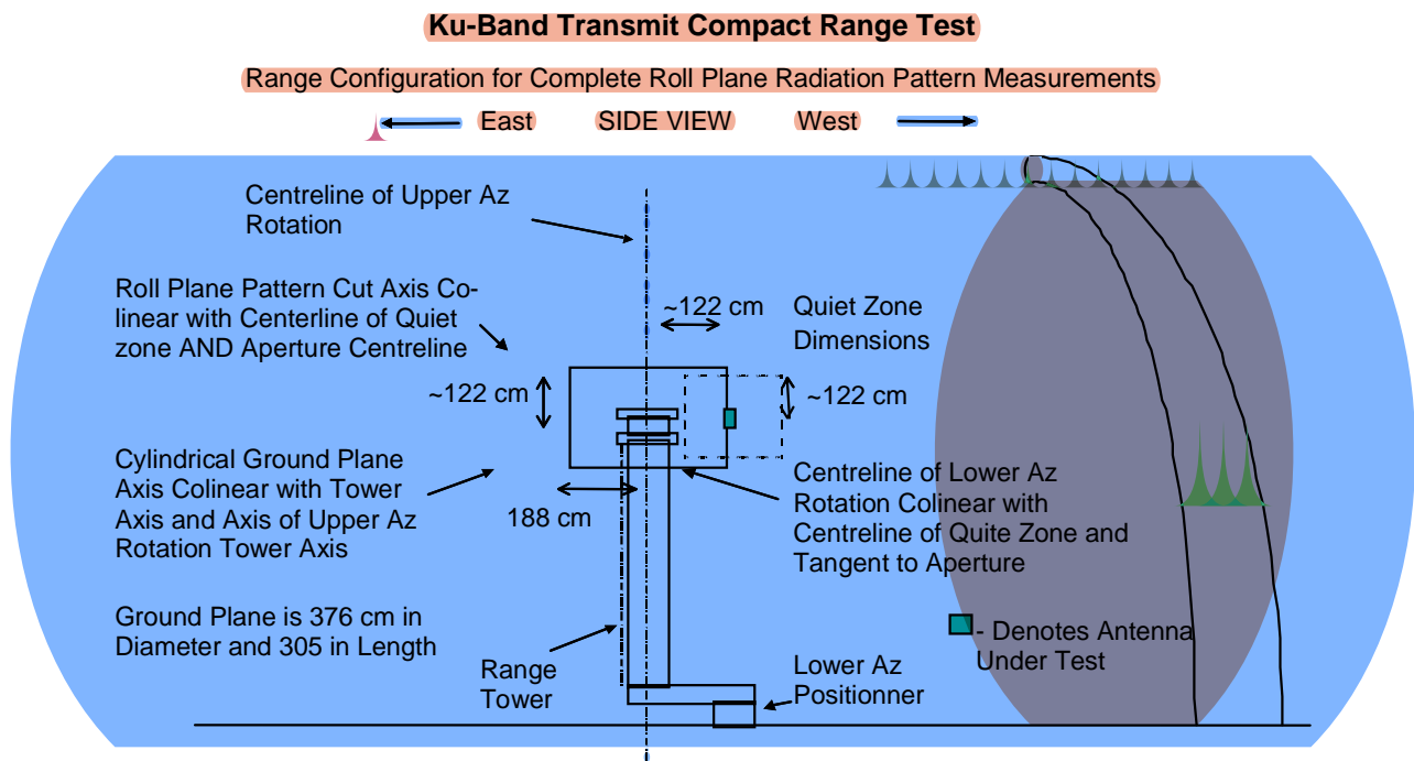
Figure 13: An example of a test set-up for measuring the roll plane radiation pattern beneath the fuselage of an aircraft
