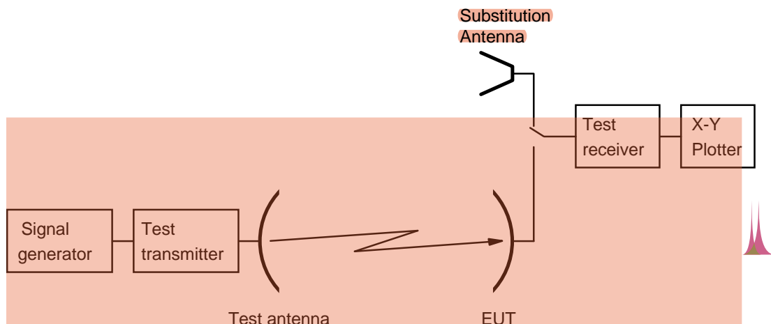
Figure 8: Test arrangement - antenna transmit gain measurement
