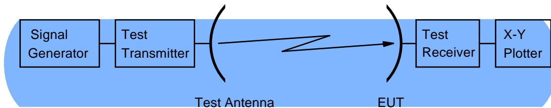
Figure 17: Test arrangement - antenna receive pattern measurement
