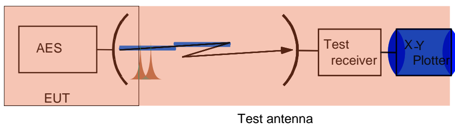
Figure 12: Test arrangement - antenna transmit radiation pattern measurement
