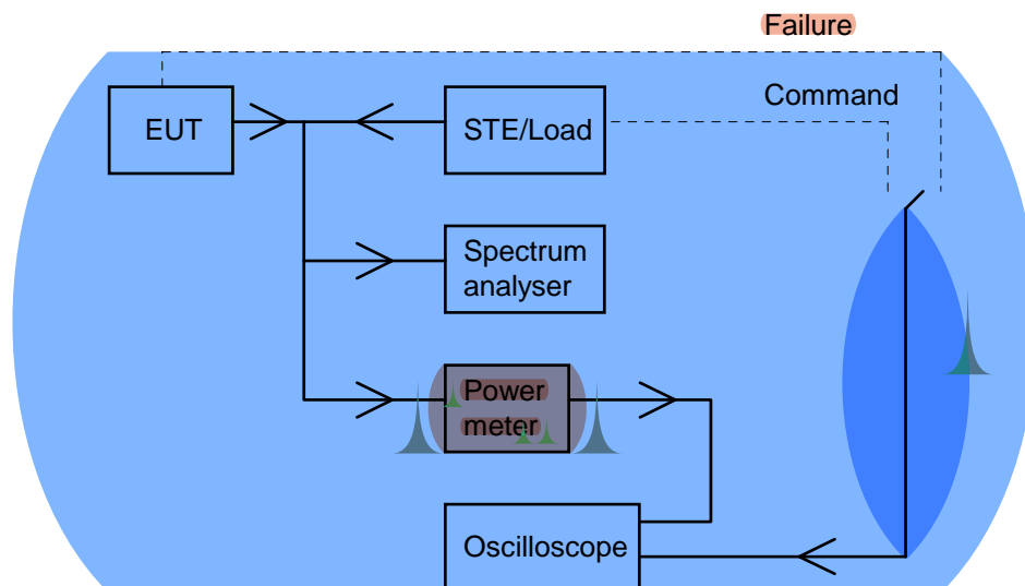
Figure 15: General test arrangement for control and monitoring tests for conducted measurements
