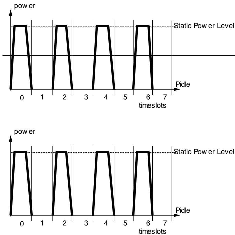
Figure 5.3.4-2: Power/time slot configuration
