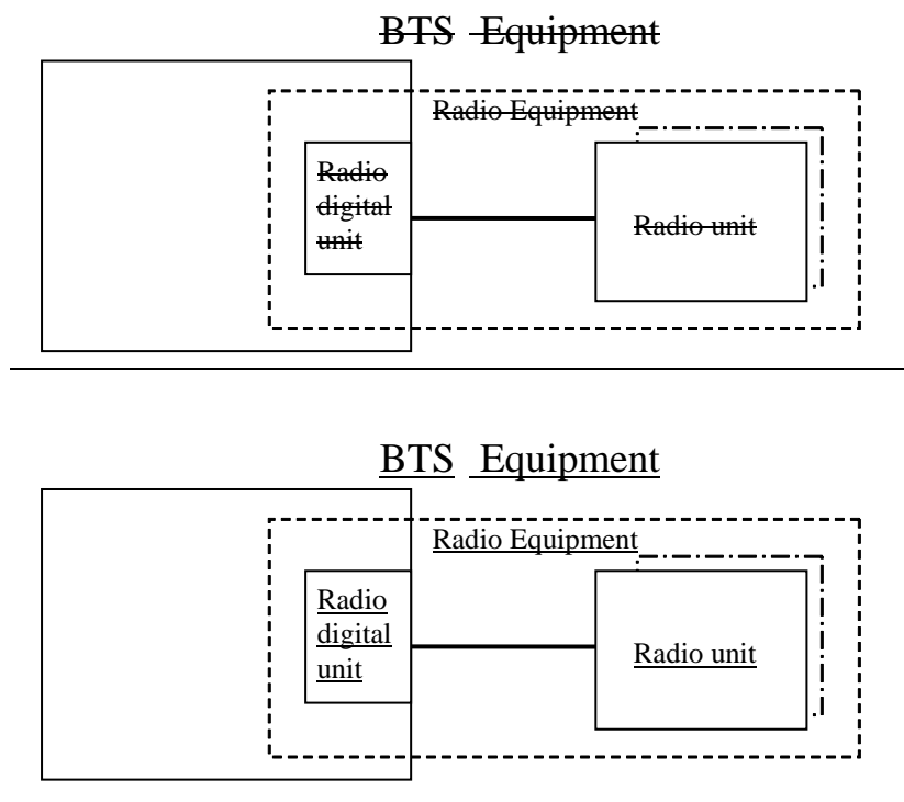
Figure 5.3.16-3: BTS with multiple enclosure solution
