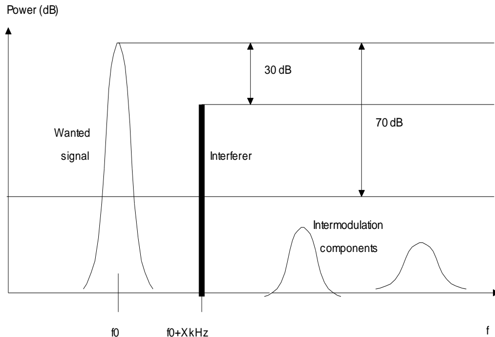
Figure 5.3.6-1: Example of TX intermodulation attenuation
