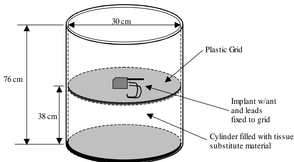
Figure C.1: Test fixture
