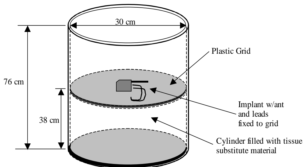
Figure BC.1: Test fixture
