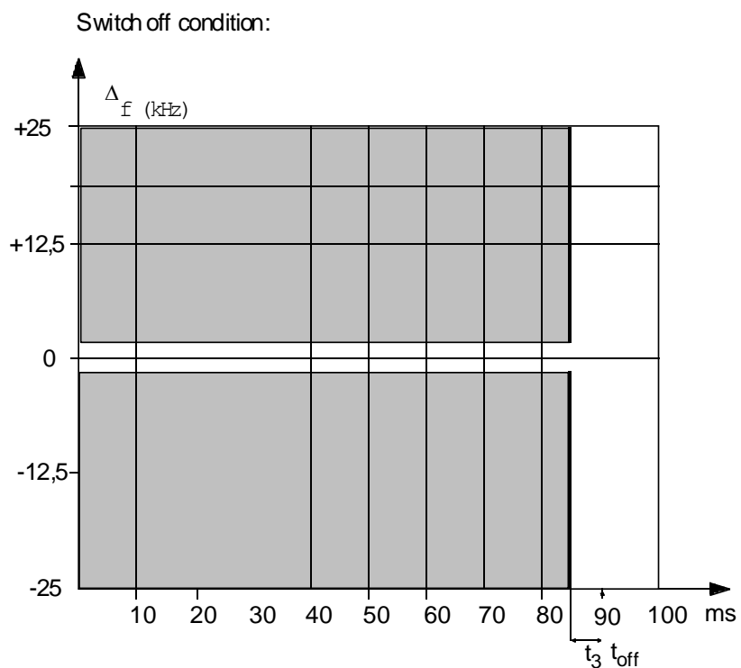
Figure 4: Storage oscilloscope view t_1 , t_2 and t_3
