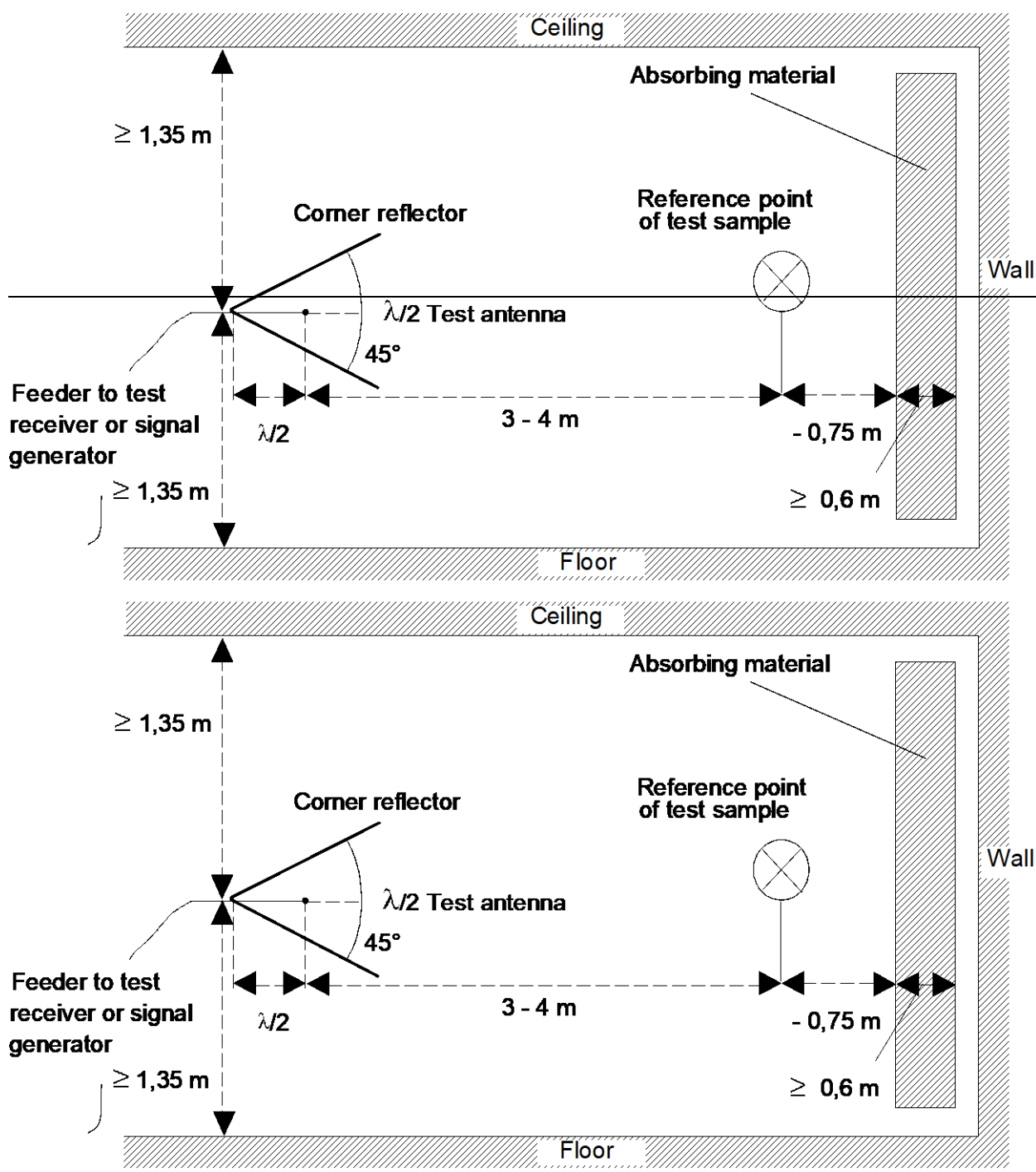
Figure AB.2: Indoors site arrangement (shown for horizontal polarization)
