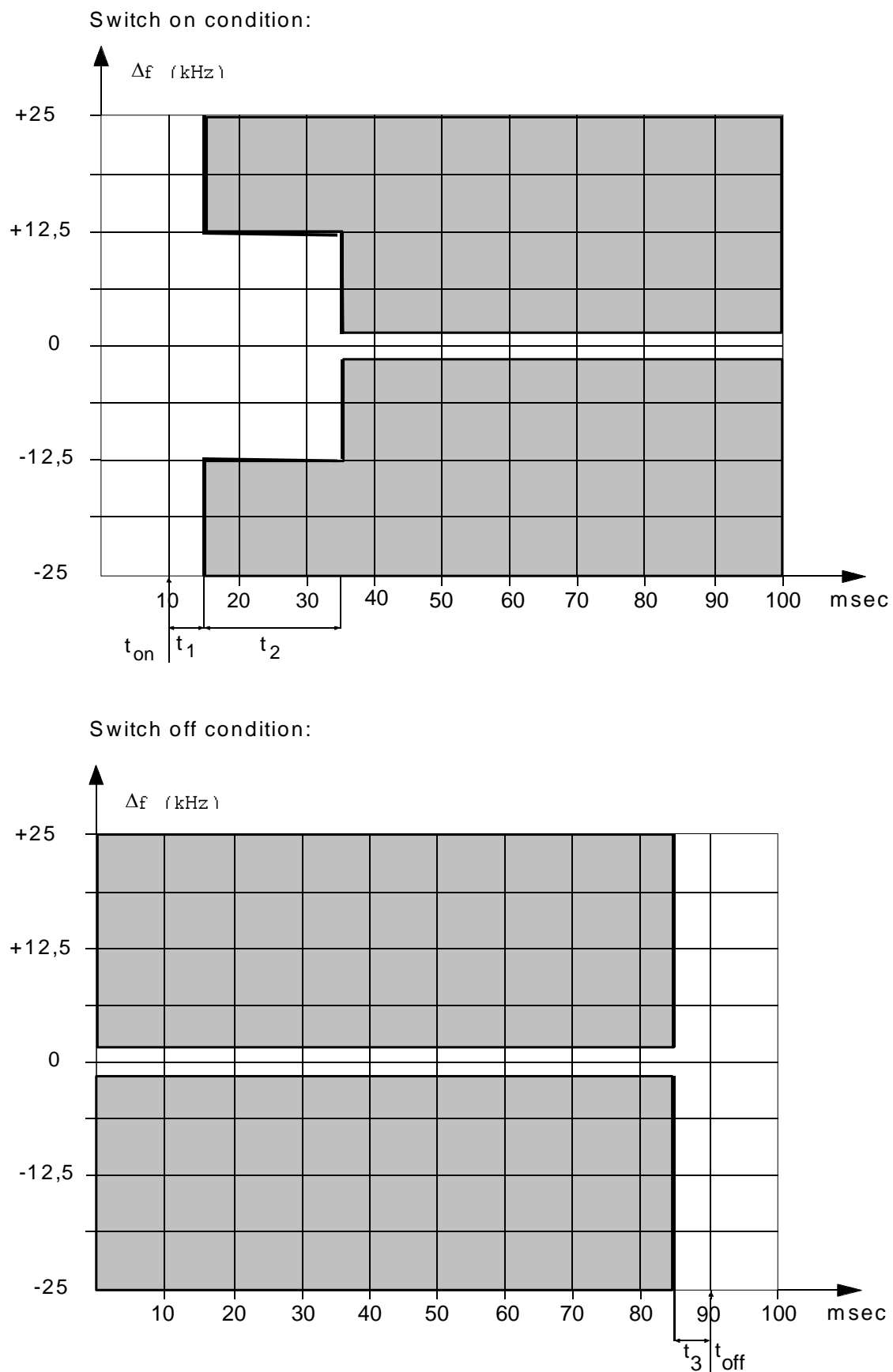
Figure 4: Switch on/off conditions
