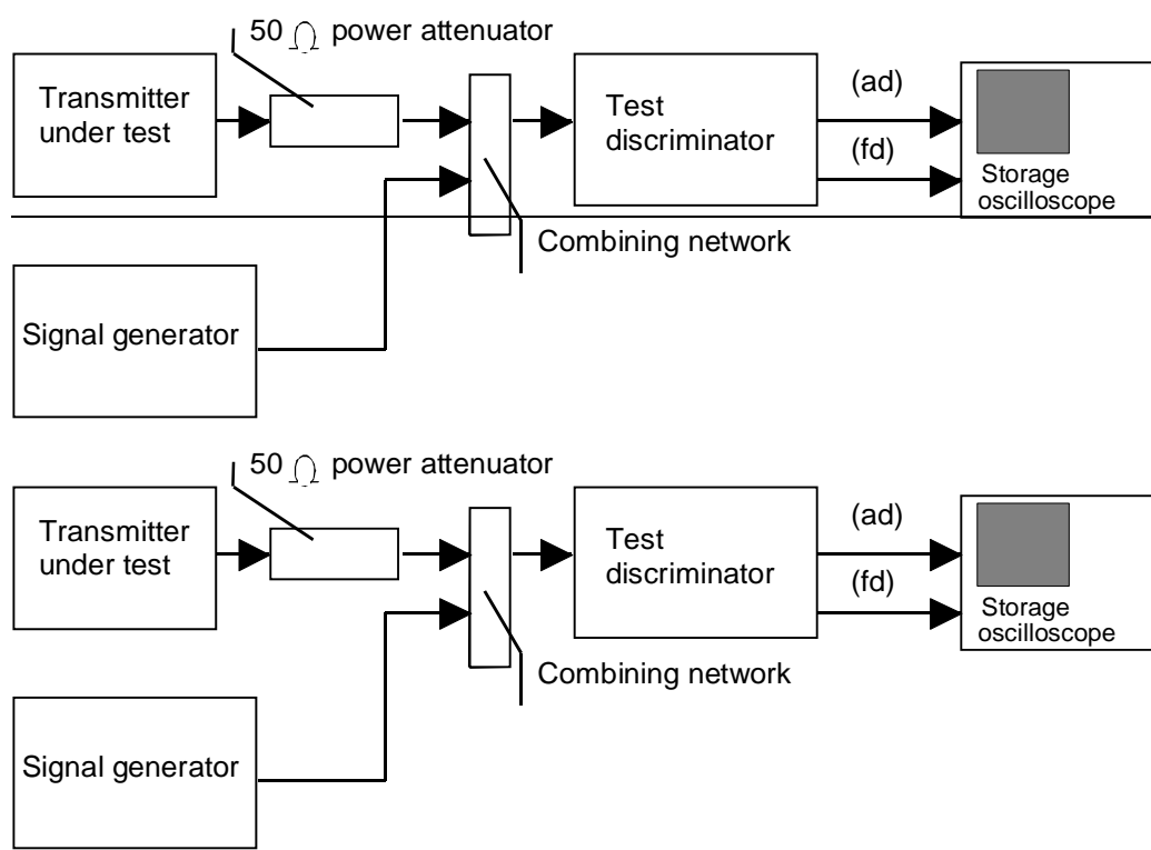
Figure 3: Measurement arrangement
