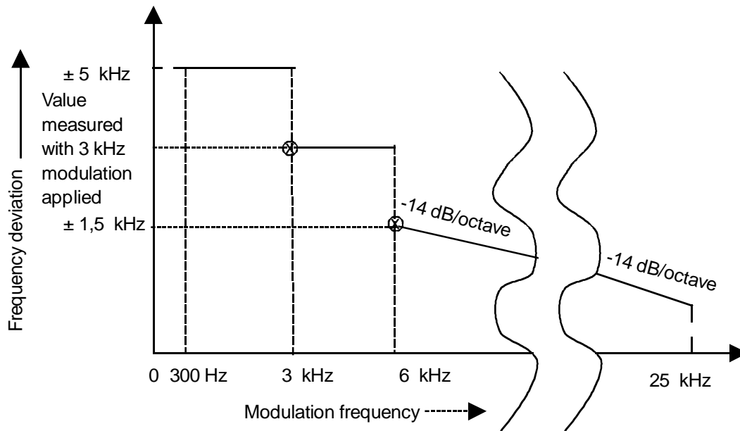
Figure 1: Frequency deviation limits
