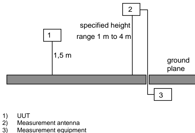
Figure C.1: Measurement arrangement No.1
