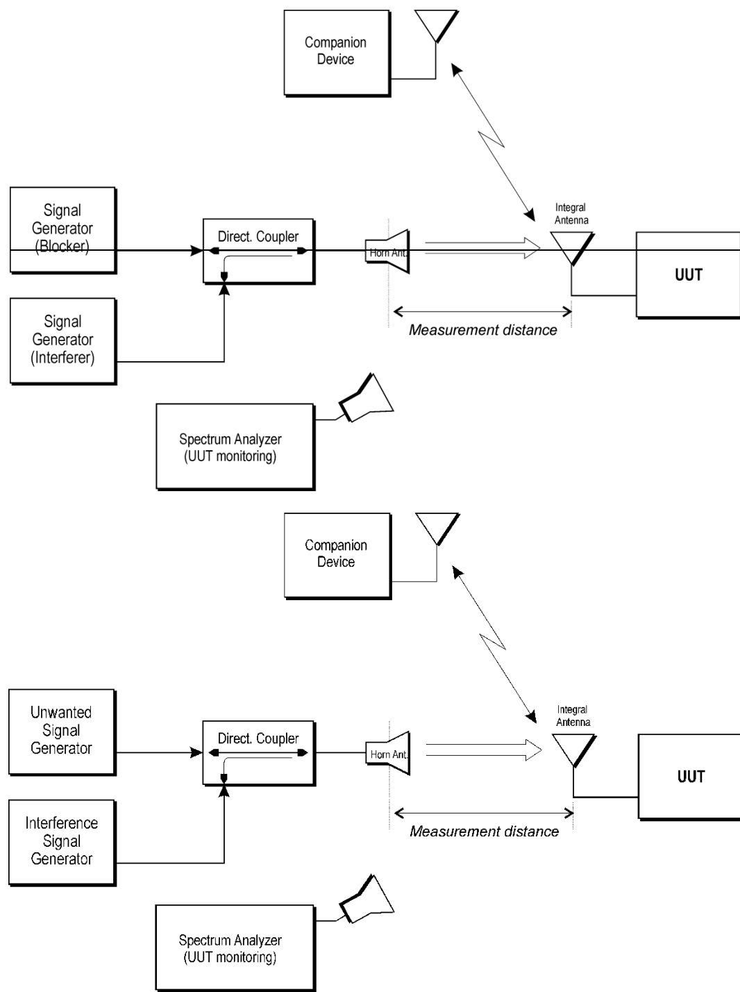
Figure C.2: Measurement Set-up
