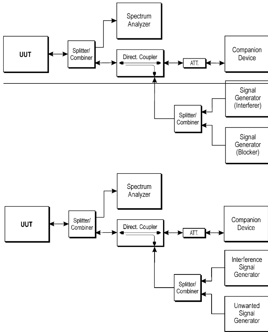
Figure 5: Test Set-up for verifying the adaptivity of an equipment
