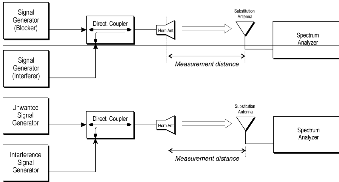
Figure C.3: Measurement Set-up - Calibration
