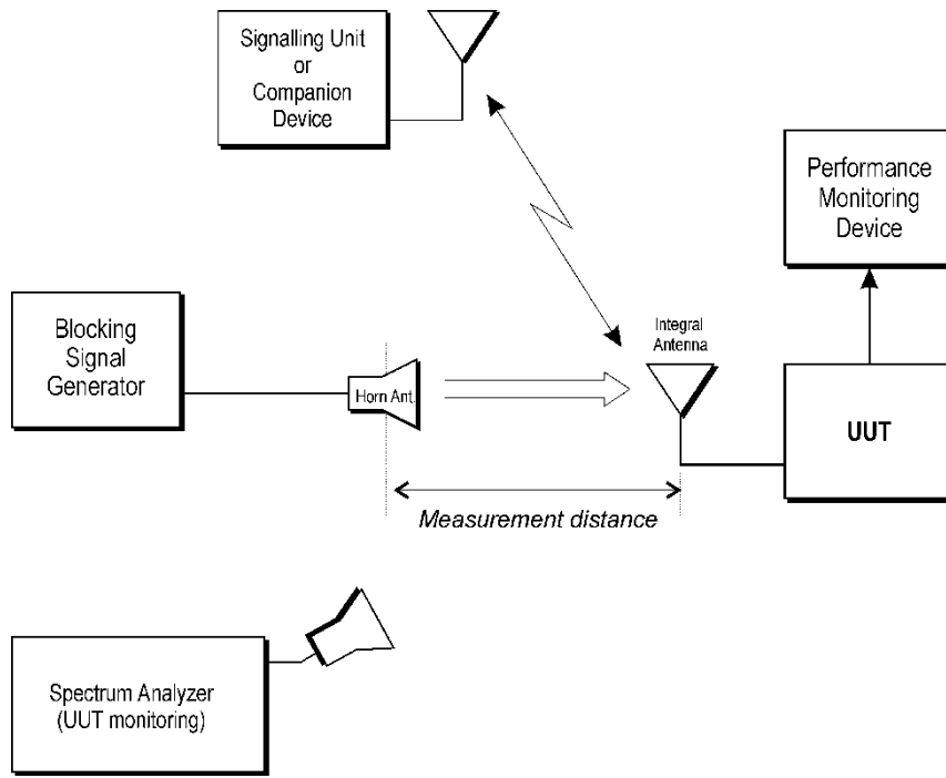
Figure C.4: Measurement Set-up
